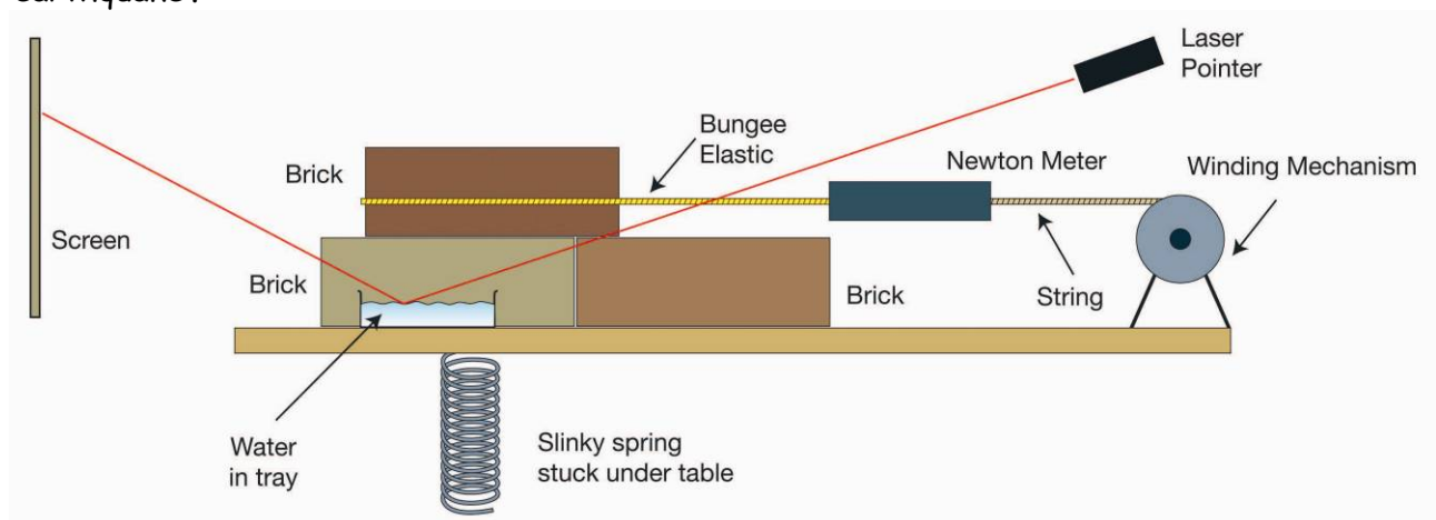
Diagram of brickquake apparatus (©ESEU)
